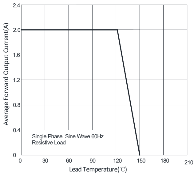
FIG1: Io-TL Curve
